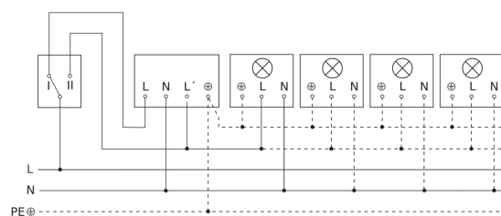
Circuit diagram Connection via a changeover switch for continuous and automatic operation
